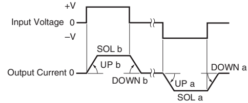
[Delay Function]
