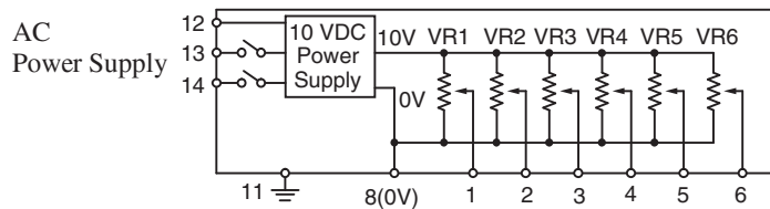
[Electric Circuit]
