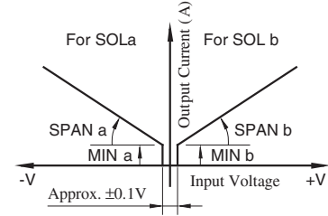
[Input-Output Characteristics]
